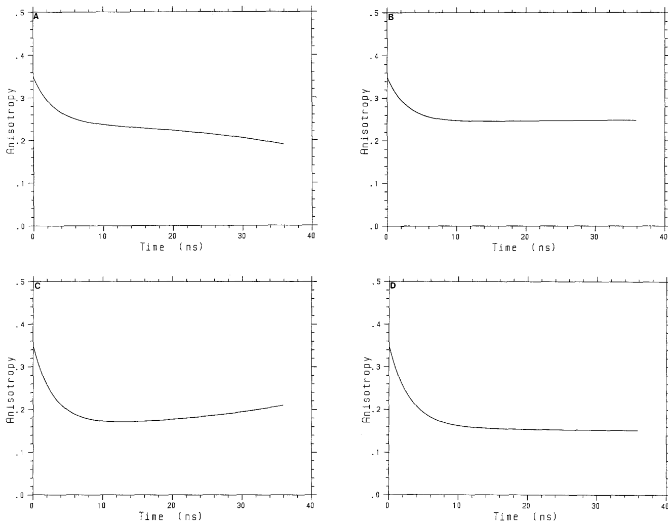
Fig. 1A–D. Simulations of the time dependence of the fluorescence anisotropy as described by (8), using the following parameters: C=0.1 , \phi_f=3.0 ns, \phi_b=2.3 ns and r(0)=0.35 . The simulations are carried out for four different combinations of \Delta\tau/\tau_f^2 and \Delta r(\infty)=r_b(\infty)-r_f(\infty)
